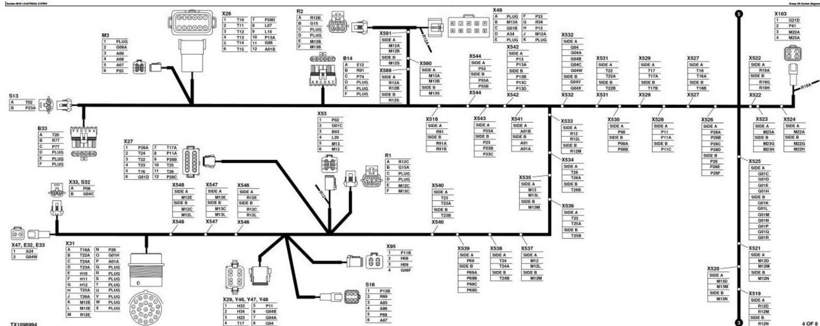
TX1000994 Lead Center Harness (M2) Wiring Diagram (1 of 8) (R.A. - 48442)
