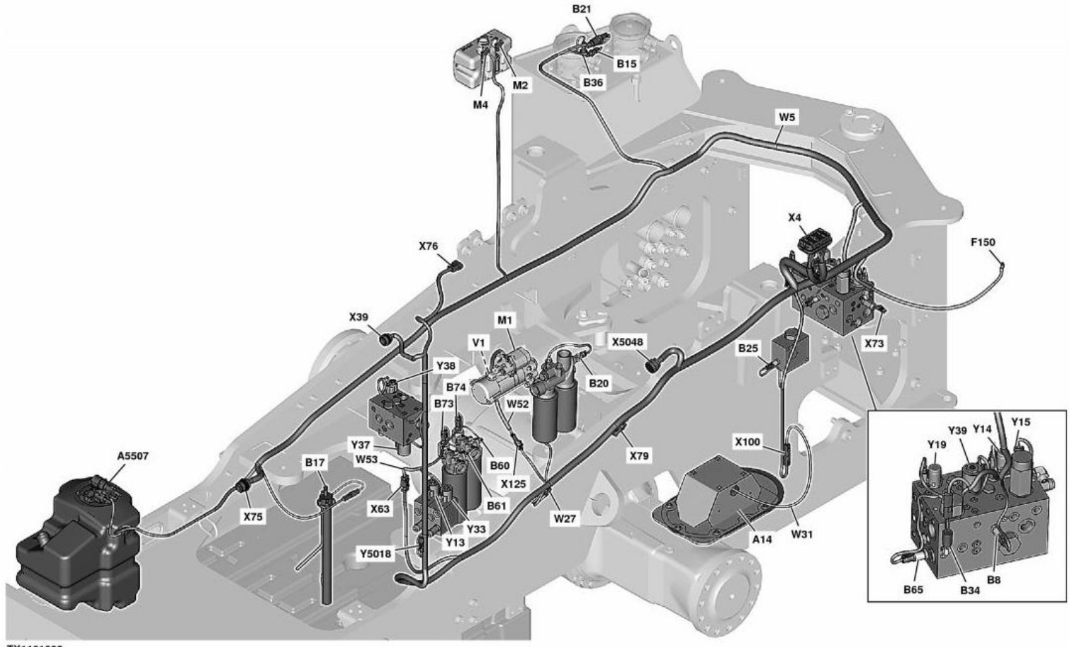
TX1161600 Engine Frame Harness (W5) Component Location
