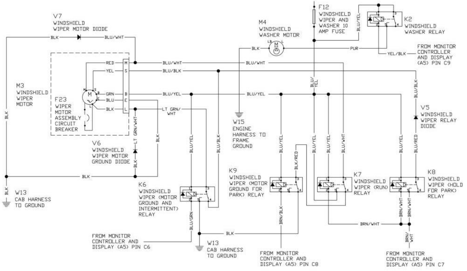
T159100 Windshield Wiper and Washer Circuit Schematic
