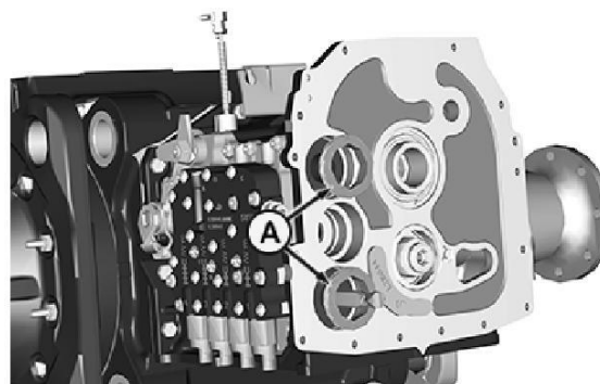
LX265509-UN: Special Nuts on Range Transmission
