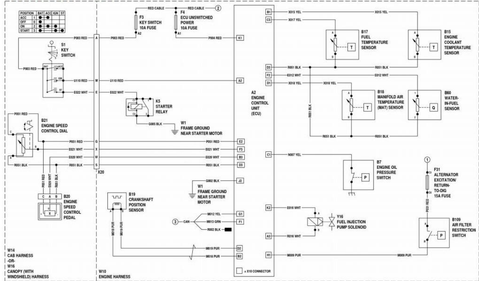
TX1138277 Engine Control Unit (ECU) Circuit Schematic (S.A. -000470)
