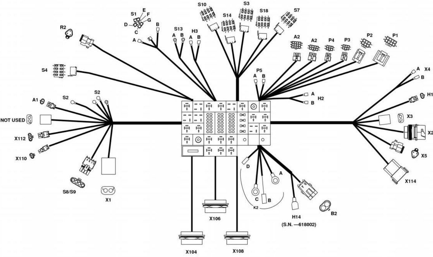
TX1044394 Fuse/Relay Wiring Harness
