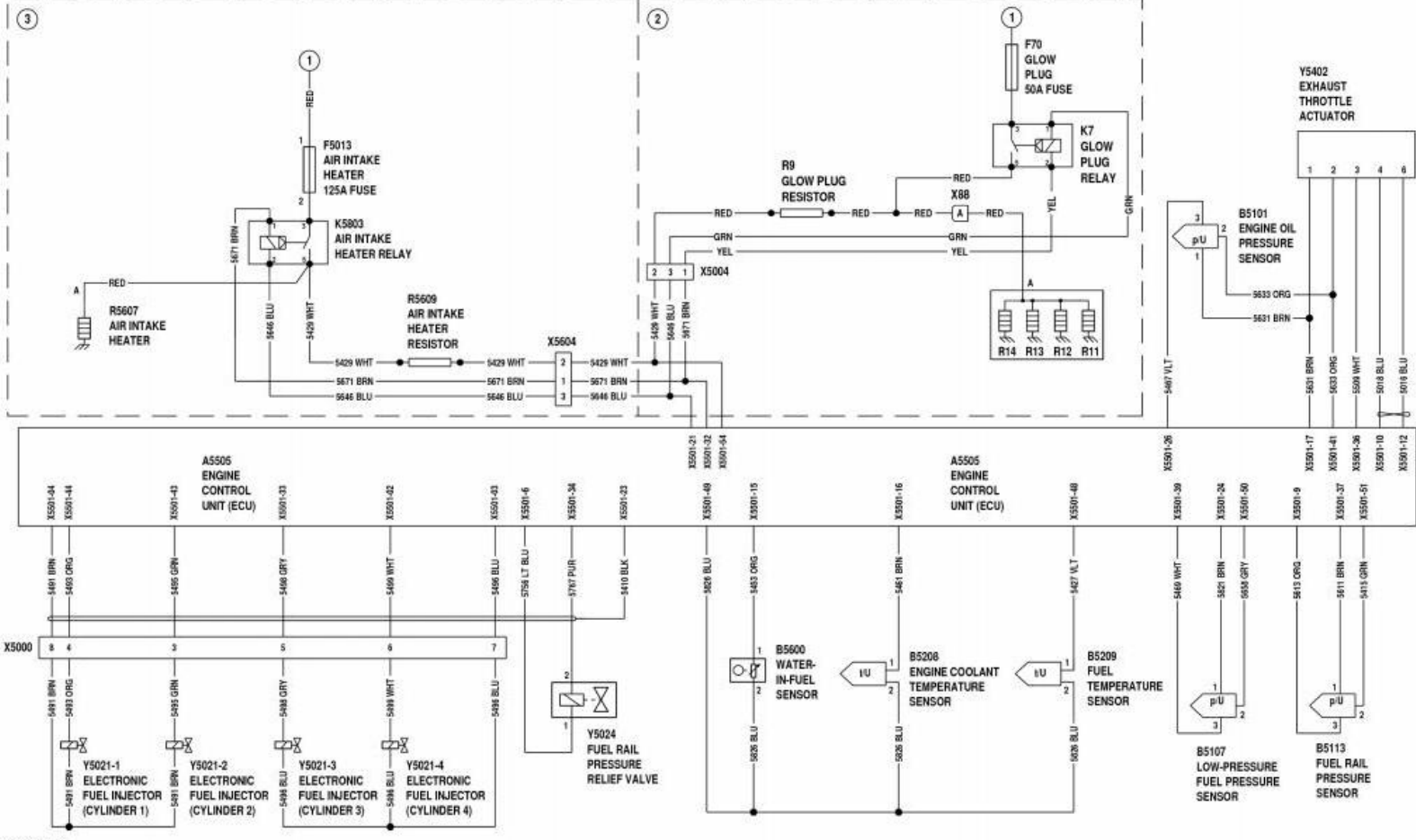
TX1184950 Engine Control Unit (ECU) Circuit Theory of Operation Schematic (2 of 4)
