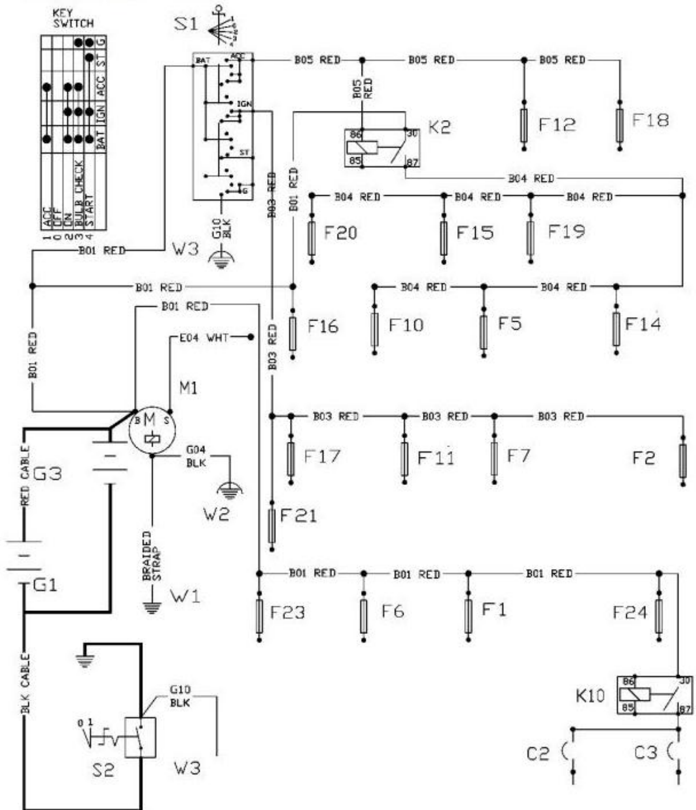
Power Circuit Schematic
