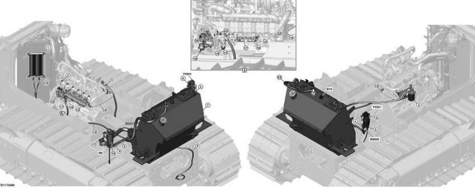
TX1174200 Engine Fuel System Component Location
