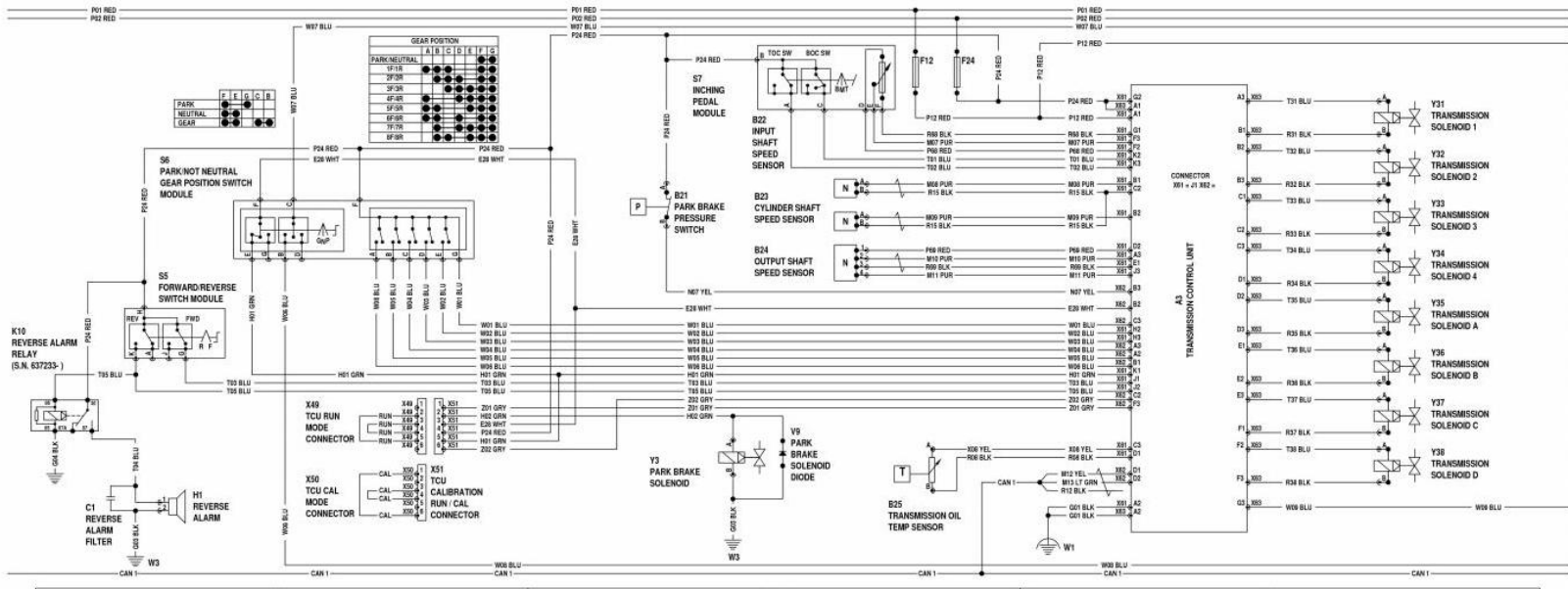
TX1099393 G AND GP SERIES MOTOR GRADER SYSTEM FUNCTIONAL SCHEMATIC (3 OF 10)
