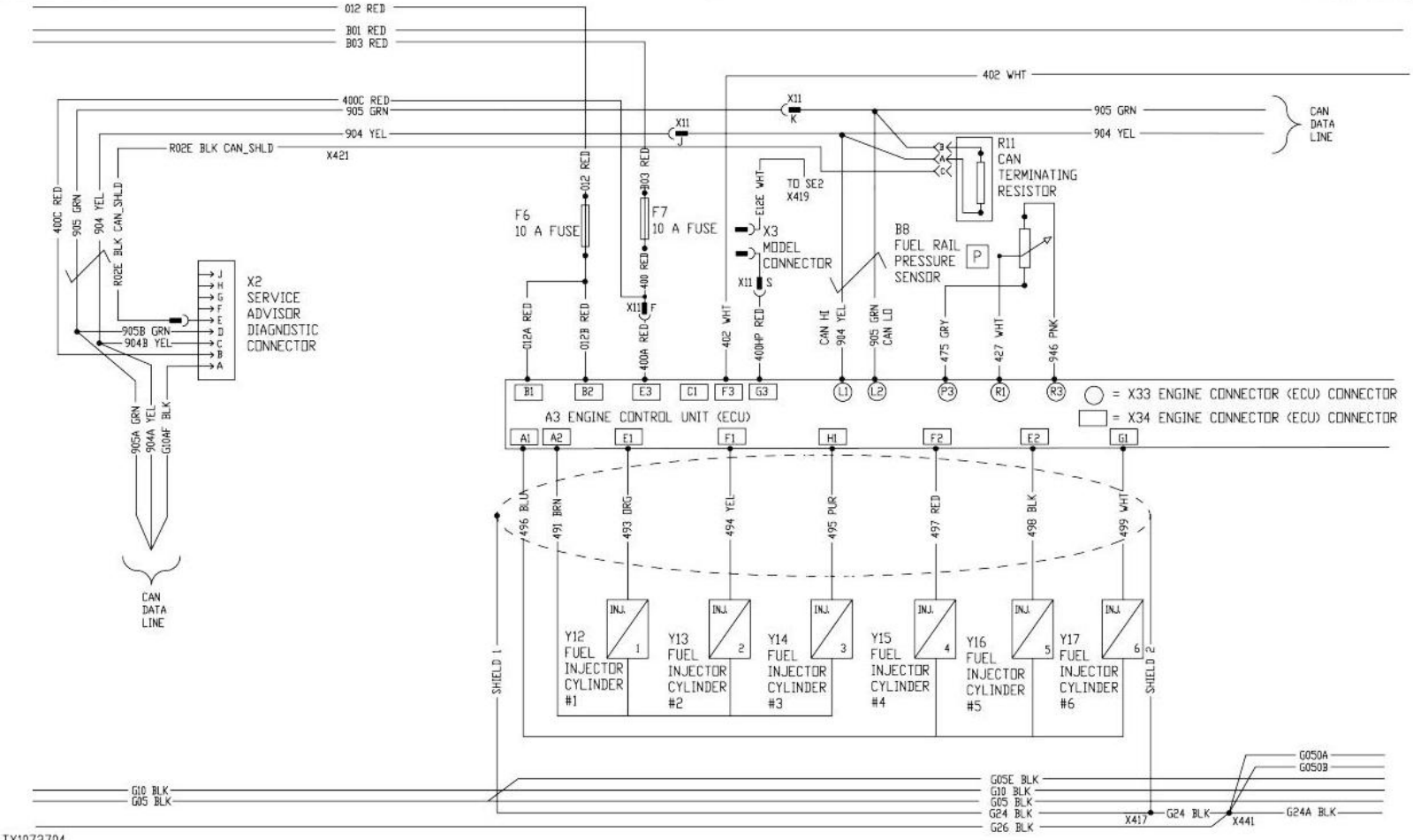
TX1072704 Engine Control Unit (ECU) Circuit Schematic (1 of 2)
