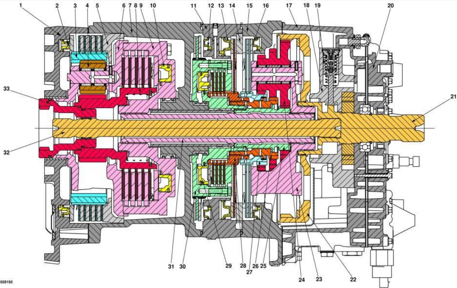
PowerQuad Module—Sectional View
