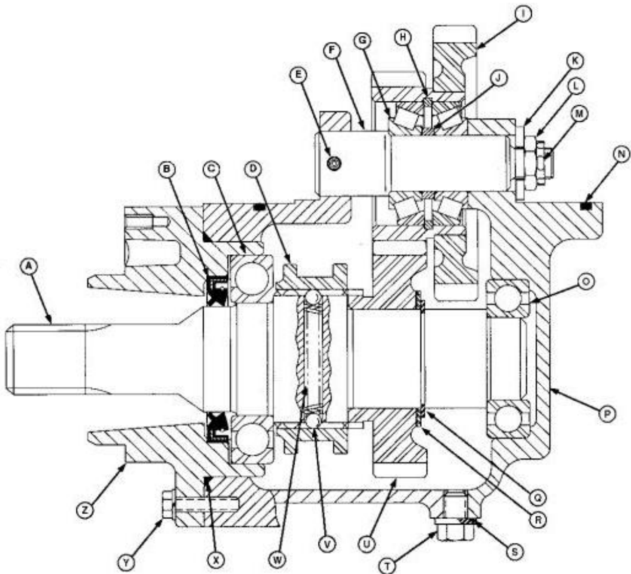
MFWD Housing Cross Sectional View
