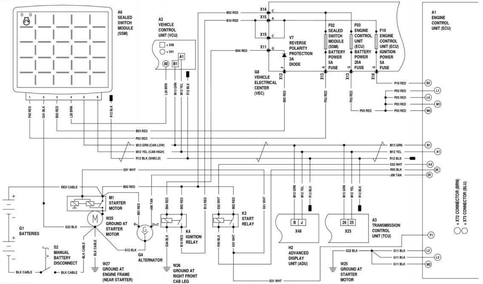
TX1106533 Engine Control Unit (ECU) Circuit Schematic (1 of 3)
