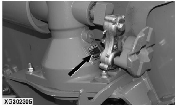
XG302305-UN: Knife Drive Gear Case—R.h Side (735PF and 740PF)
