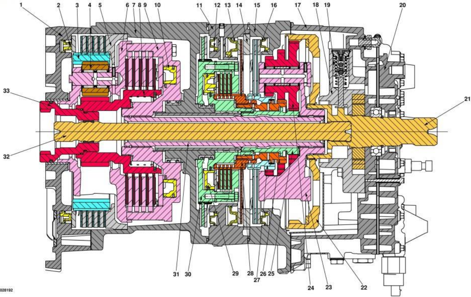
PowerQuad Module—Sectional View
