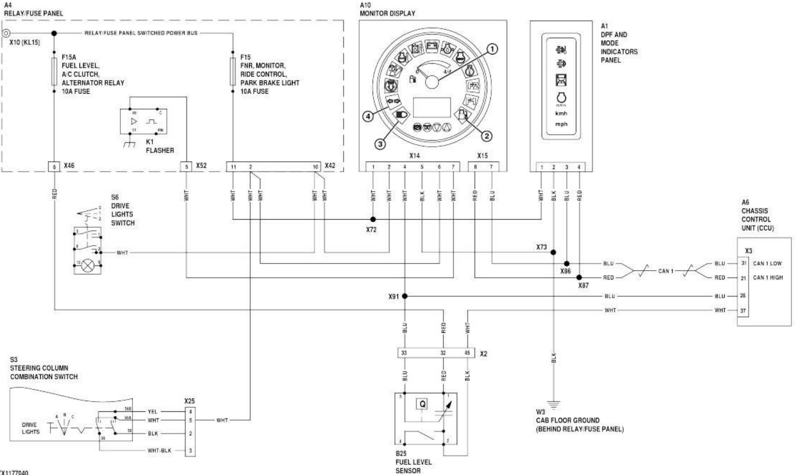
TX1177040 Monitor Display Circuit Schematic
