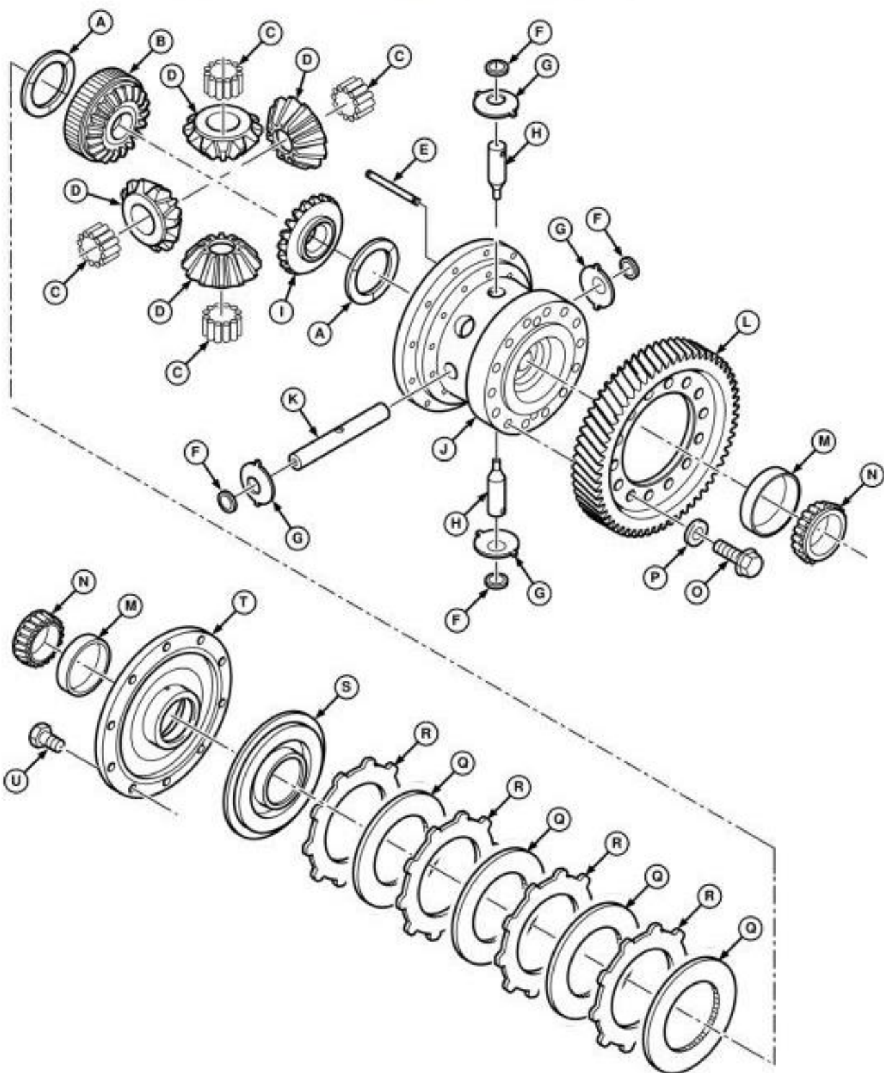
Differential Module (With Differential Lock) - Exploded View
