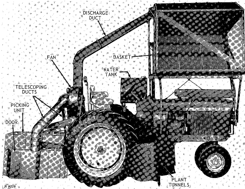
Fig. 10-5-1-11 Cotton Picker on 3010 Tractor
