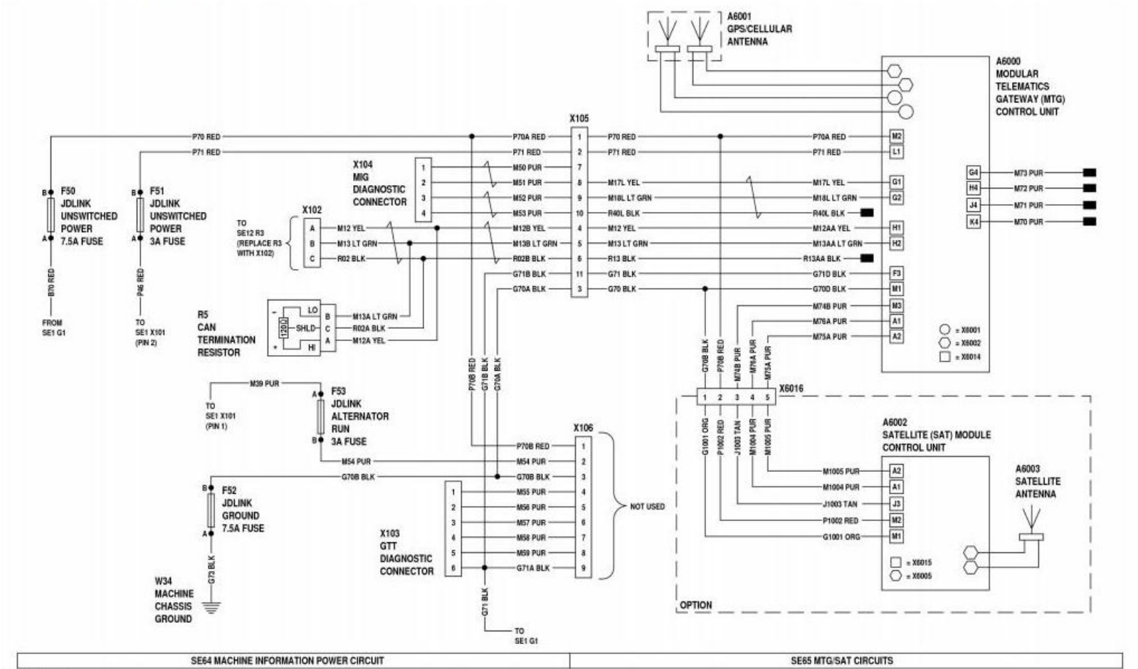
TX1144698 SE64 MACHINE INFORMATION POWER CIRCUIT SE65 MTG/SAT CIRCUITS JDLink™ Functional Schematic—MTG/SAT
