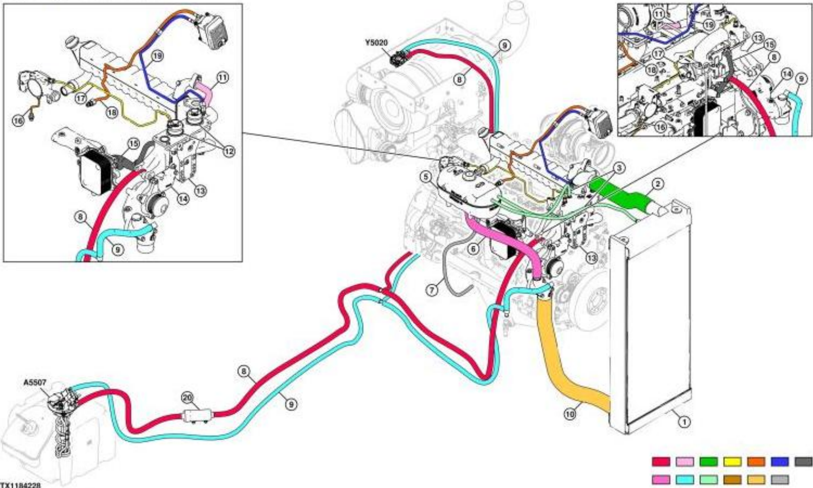
Engine Cooling System Component Location
