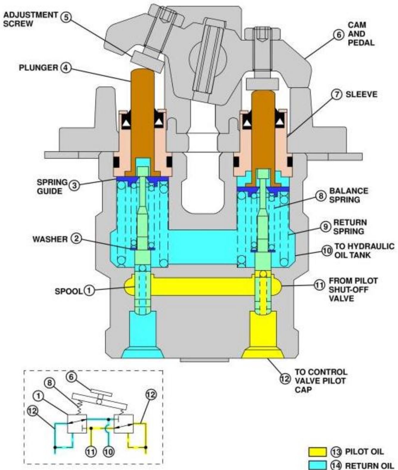
15 PROPEL PILOT CONTROLLER - FULL STROKE
