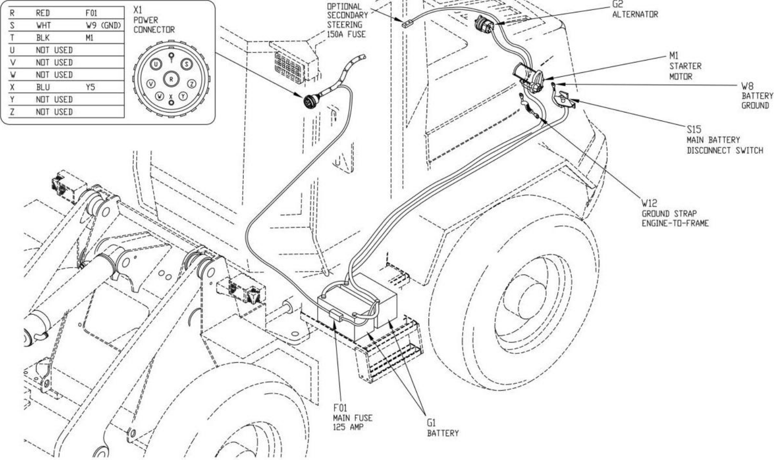
Power And Battery Cable Location
