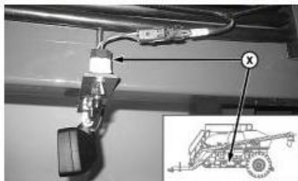
X21 — Auxillary Outlet Connector
