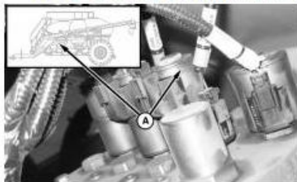
Y741 — Elevation Cylinder Retract Solenoid Valve
