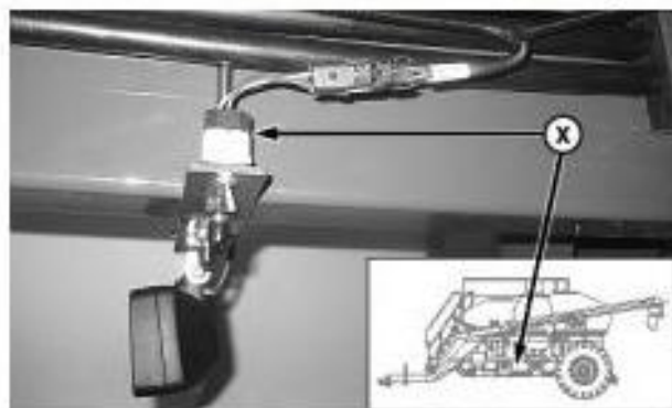
X20 - ON / OFF Fill Switch
